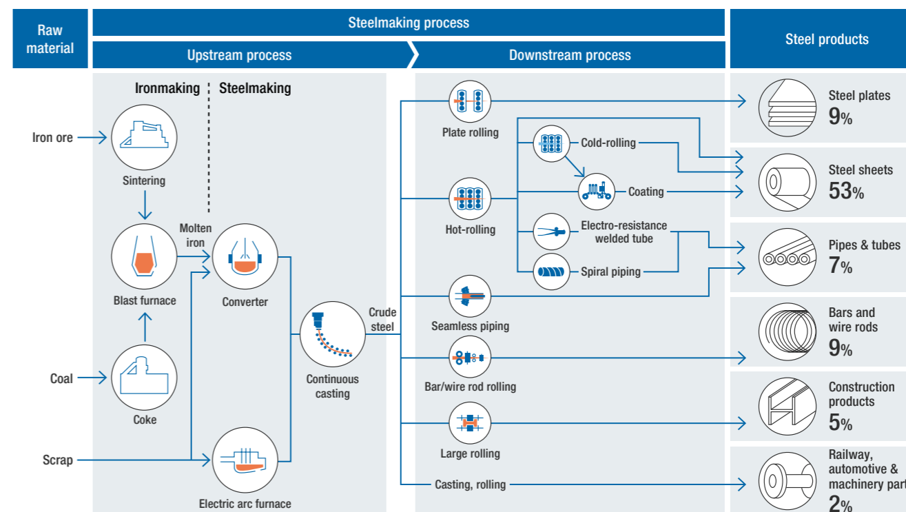
Steel product manufacturing process
