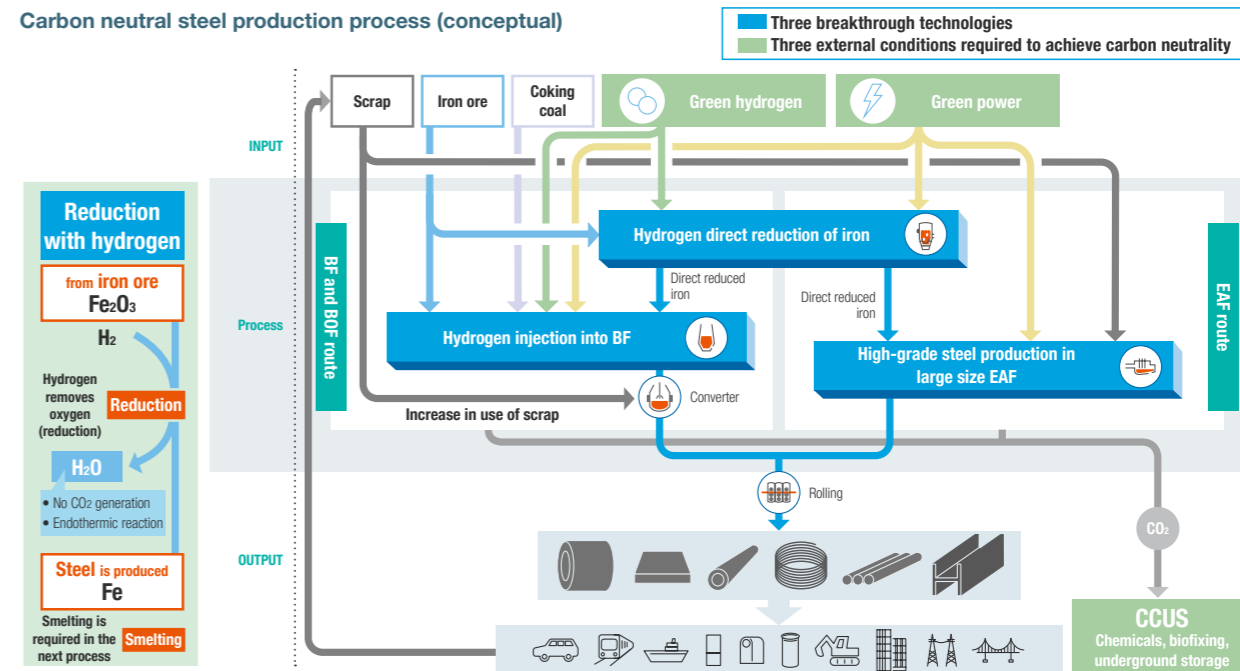
Carbon neutral steel production process (conceptual)
